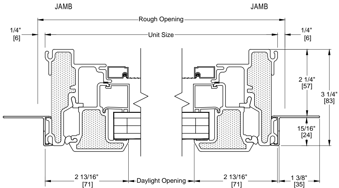
HORIZONTAL SECTION
