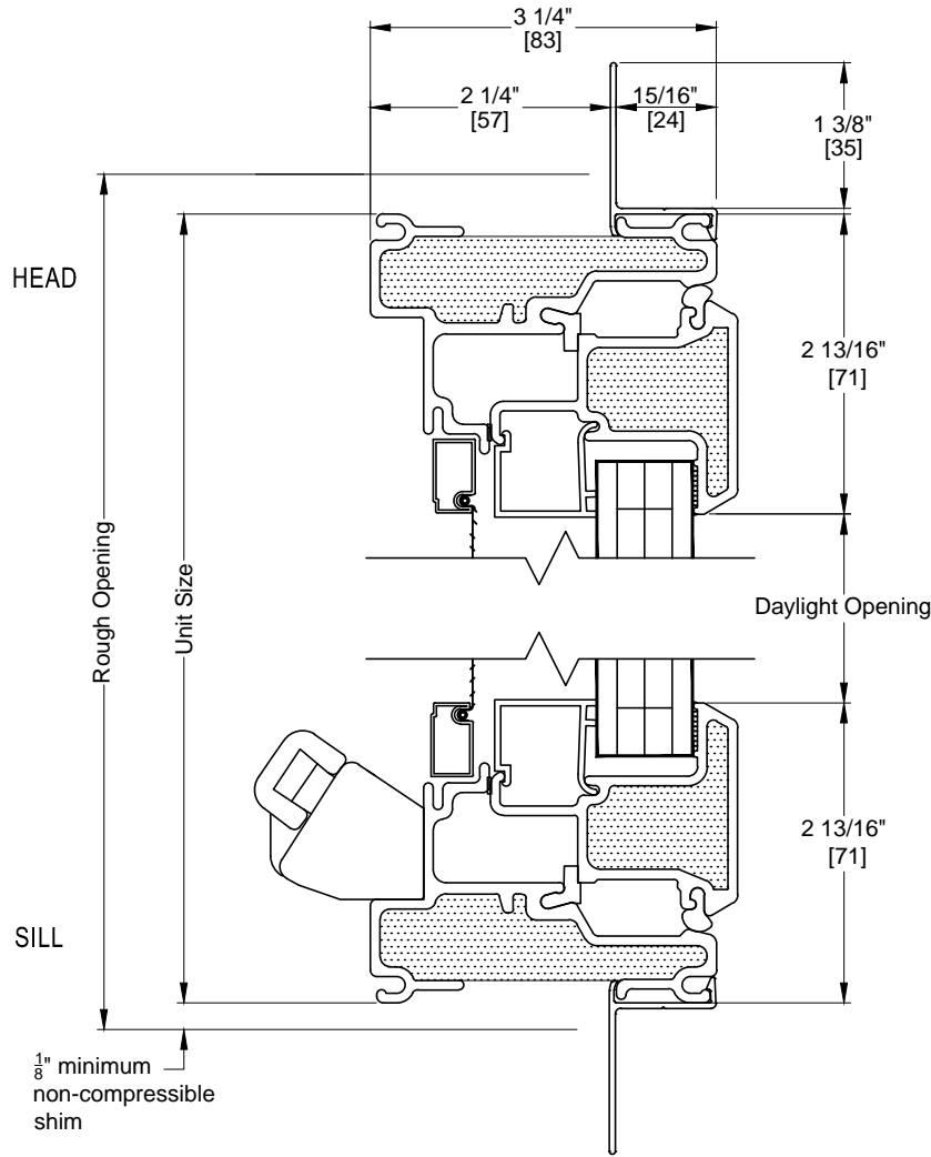
VERTICAL SECTION
