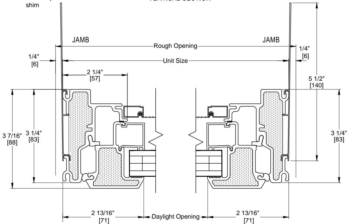
HORIZONTAL SECTION
